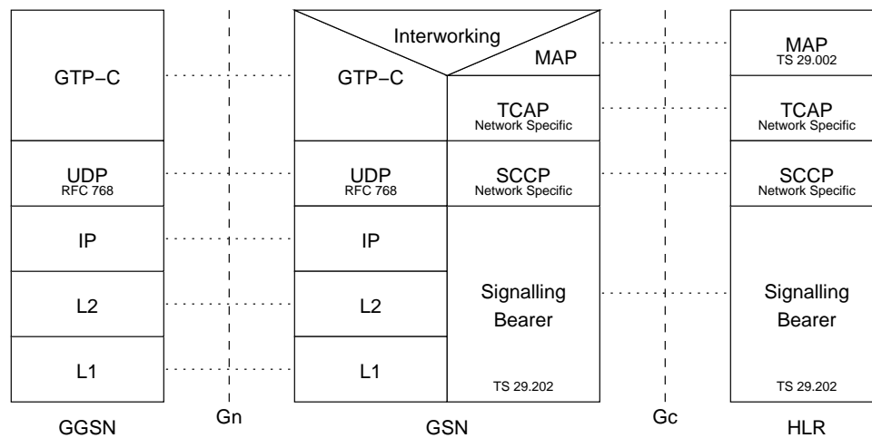
Figure 3.7: Gn/Gc Interface
