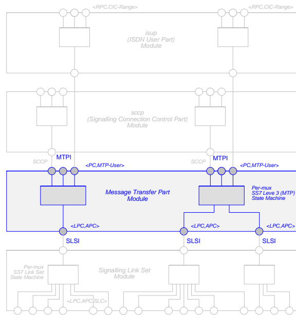
Figure 6.4: Message Transfer Part (MTP) Level 3 (MTP3) Module
